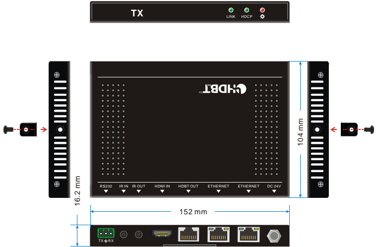
5-1 Transmitter
