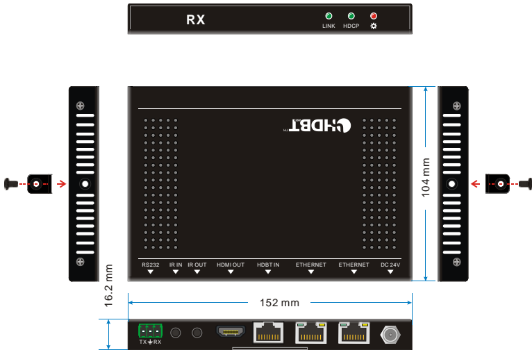
5-2 Receiver
