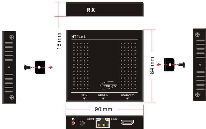
5-2 Receiver (TP70LR)
