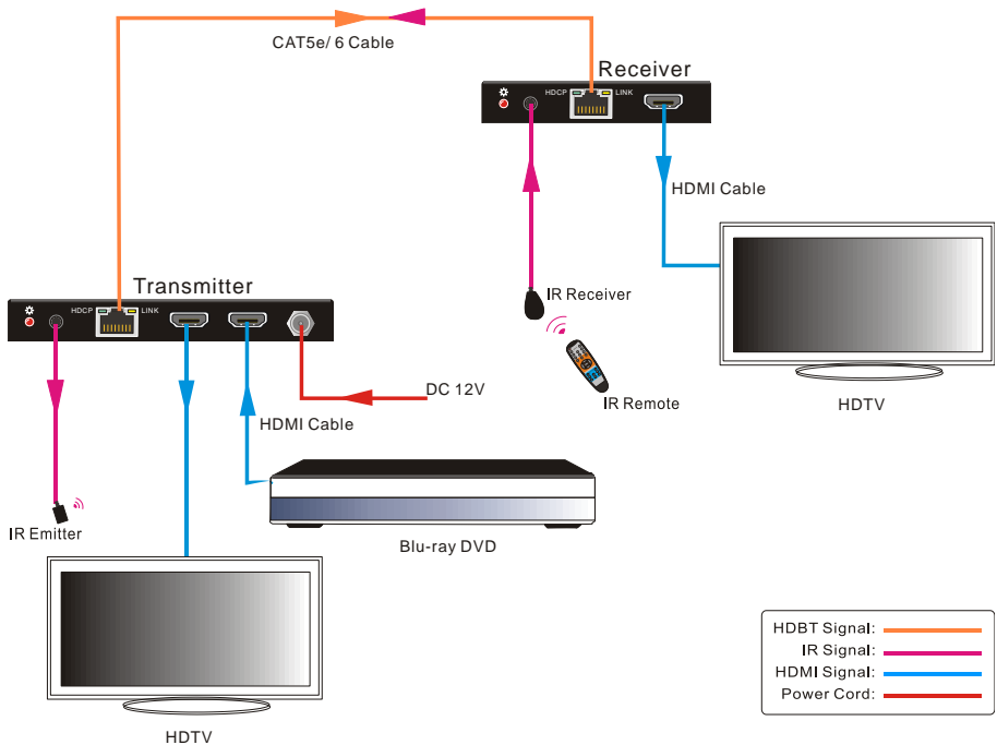
Figure 3- 1 System Connection
