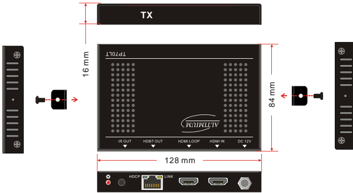
5-1 Transmitter (TP70LT)
